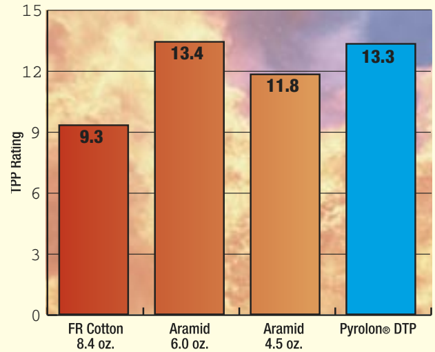
Thermal Protective Performance-Spaced
