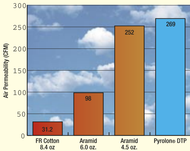
Air Permeability
