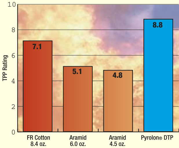
Thermal Protective Performance-Contact
